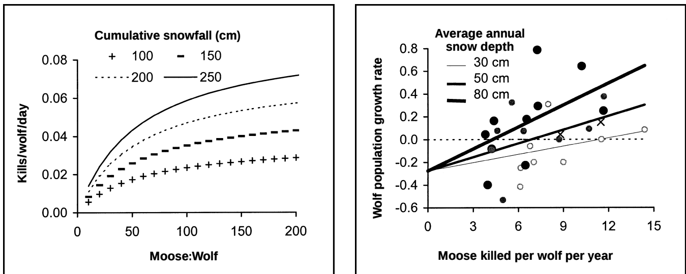
Figure 10. (Left) Wolves kill more moose (y-axis) during years when there are more moose per wolf (x-axis). These relationships, called functional response and numerical response, together determine the nature of predator-prey dynamics. Winter climate has an important impact on both relationships. In years with more snow, wolves not only kill more moose (left), they are also more efficient at converting moose killed into wolf population growth (right), possibly because moose are less fit.
