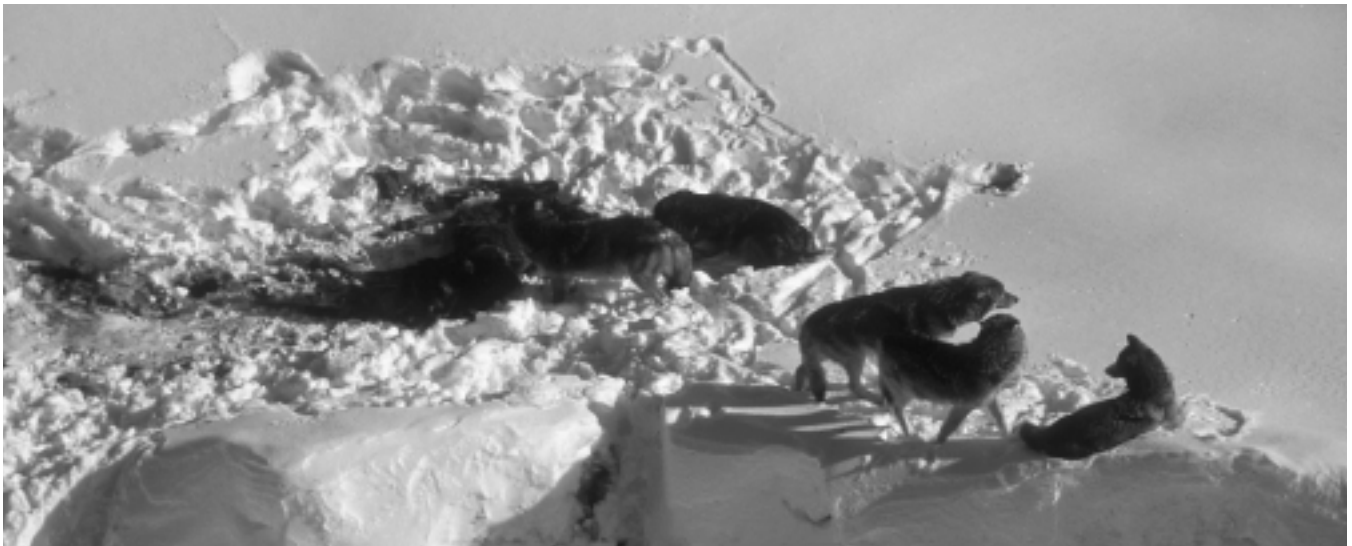
Figure 7. With deep snow in the interior, the shorelines of Isle Royale were primary travel routes and kill sites for wolves in winter 2001.
