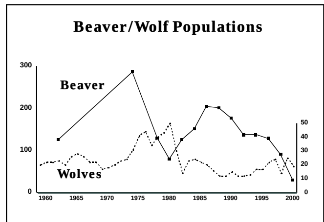
Figure 24. Beaver abundance dropped in 1980 when wolves reached a peak, but the recent decline is linked to an aging forest that is increasingly composed of coniferous tree species.
